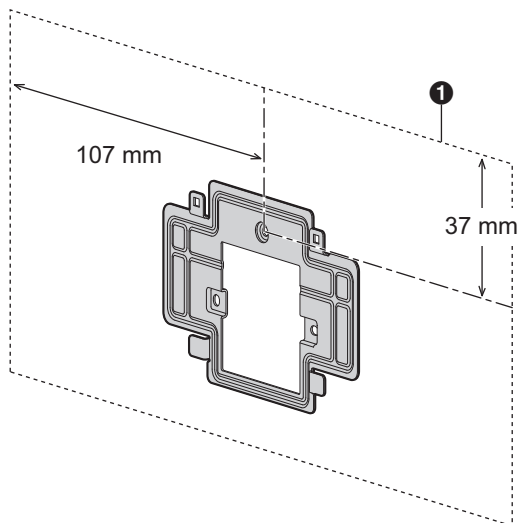
1 Room monitor installation location
